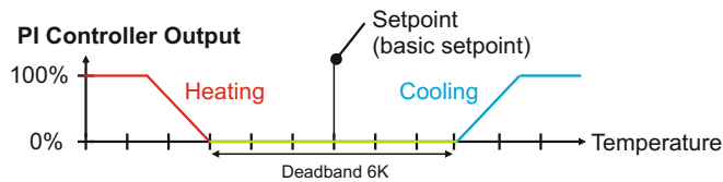
Lowering Mode
